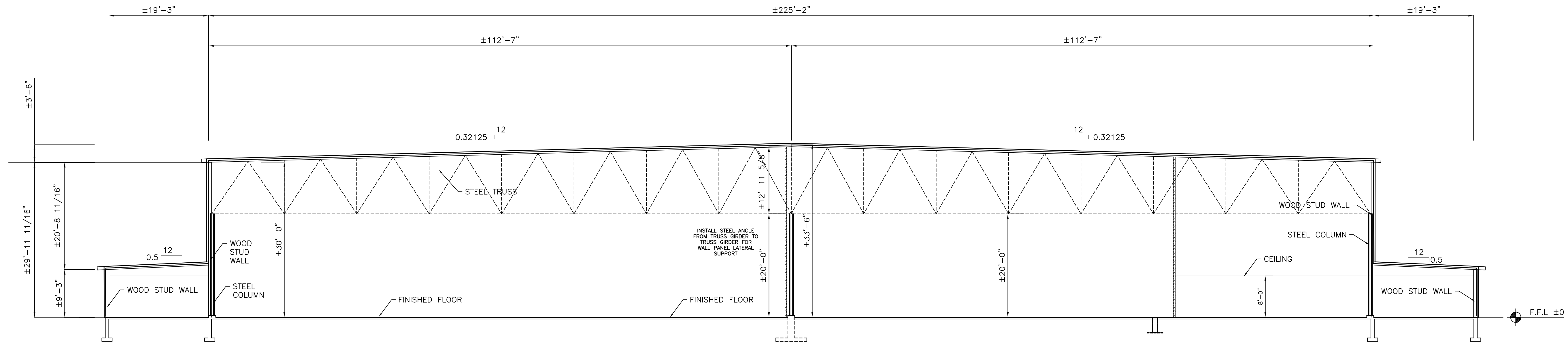
A-A CROSS-SECTION SCALE 1/8" = 1'-0"
