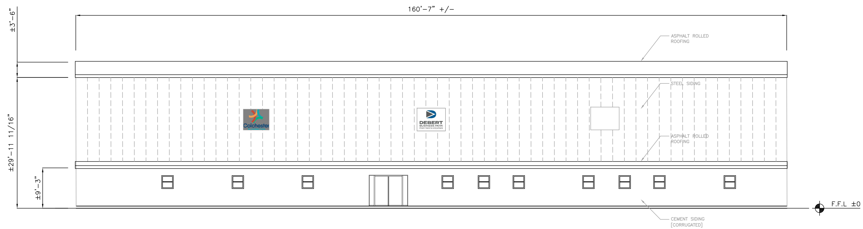
2 A101 SIDEWALL ELEVATION - EAST SCALE 1/8" = 1'-0"
